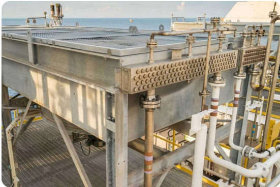
Special FinFan Maintenance Tools
